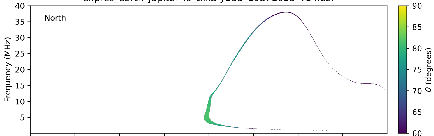
expres_earth_jupiter_io_txka-y235_19871013_v14.cdf
