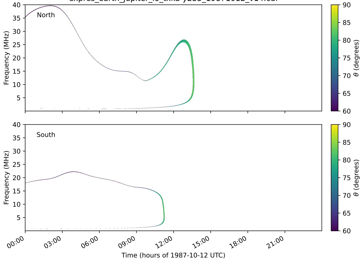
expres_earth_jupiter_io_txka-y235_19871012_v14.cdf
