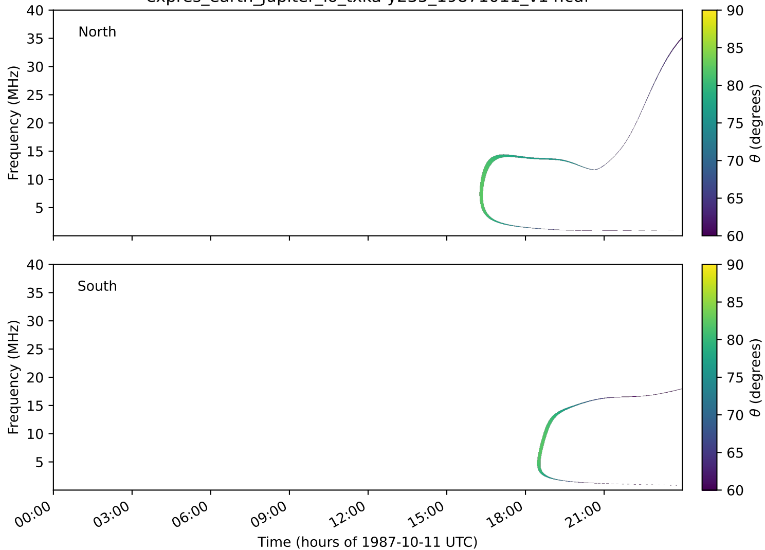
expres_earth_jupiter_io_txka-y235_19871011_v14.cdf
