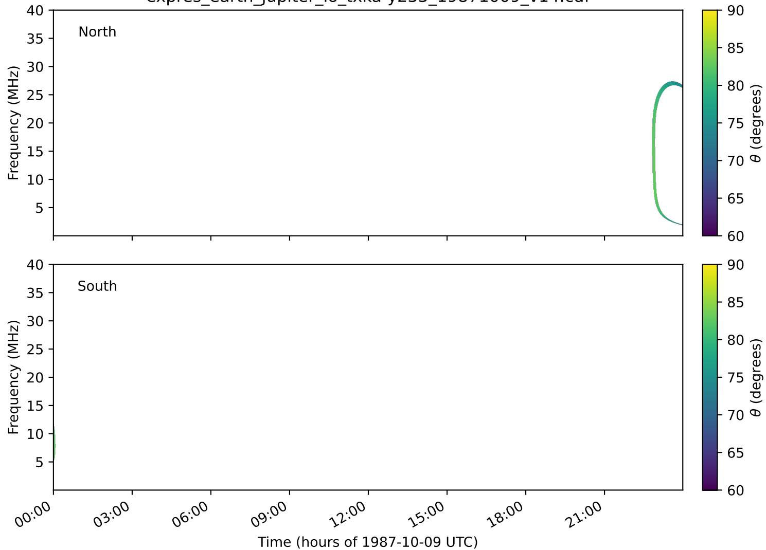
expres_earth_jupiter_io_txka-y235_19871009_v14.cdf
