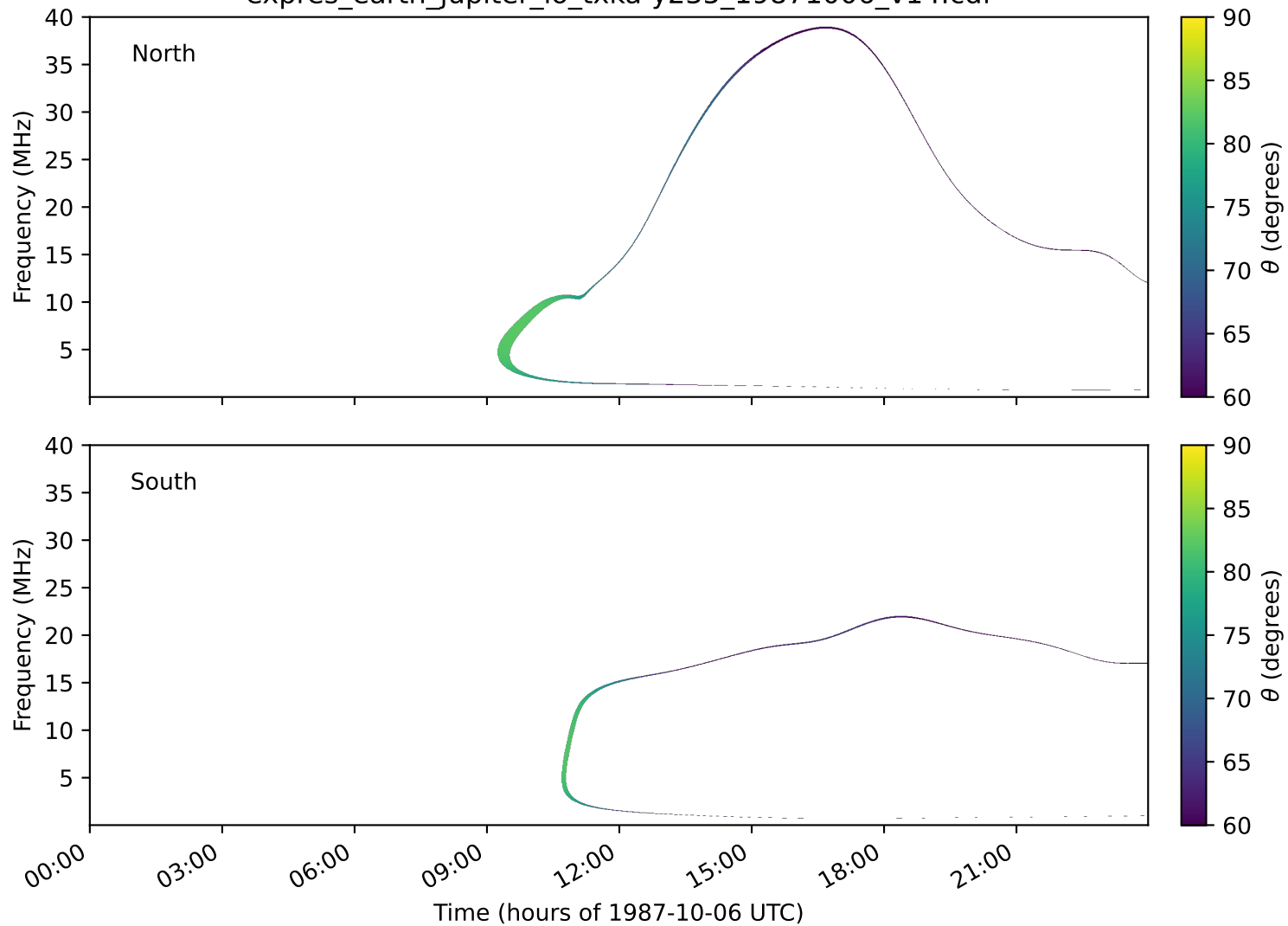
expres_earth_jupiter_io_txka-y235_19871006_v14.cdf
