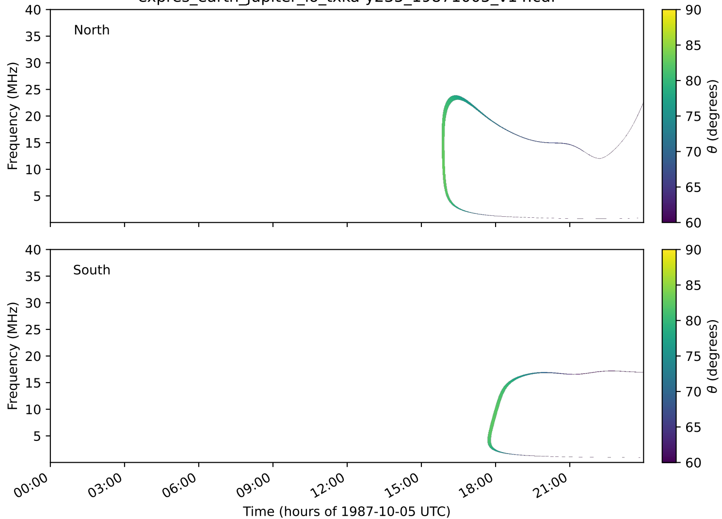
expres_earth_jupiter_io_txka-y235_19871005_v14.cdf
