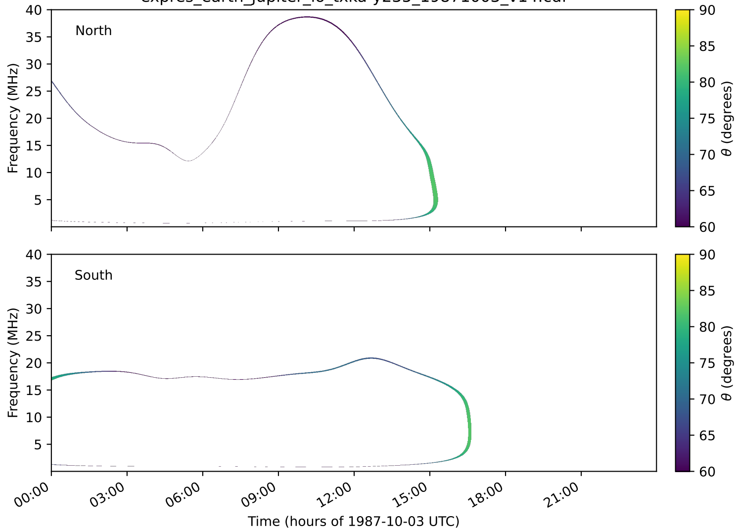
expres_earth_jupiter_io_txka-y235_19871003_v14.cdf
