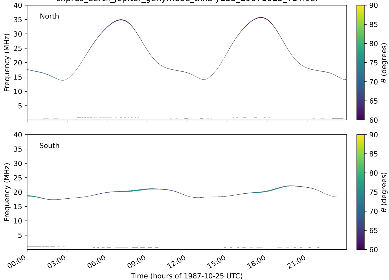
expres_earth_jupiter_ganymede_txka-y235_19871025_v14.cdf
