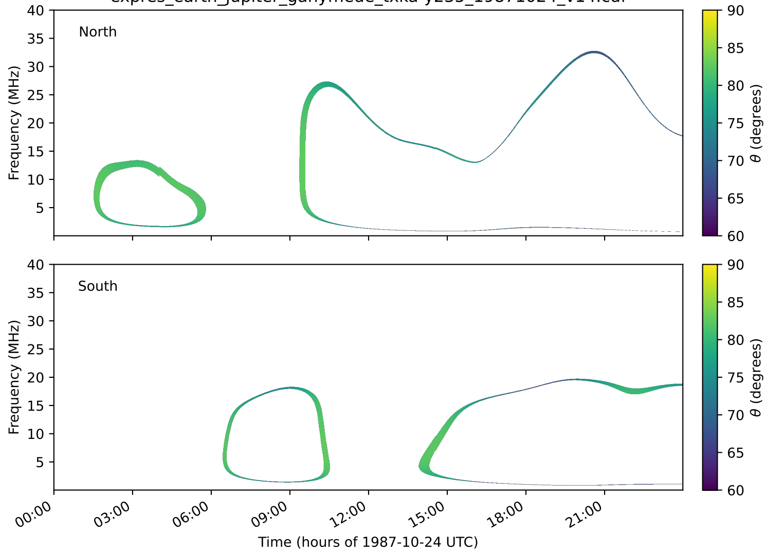
expres_earth_jupiter_ganymede_txka-y235_19871024_v14.cdf
