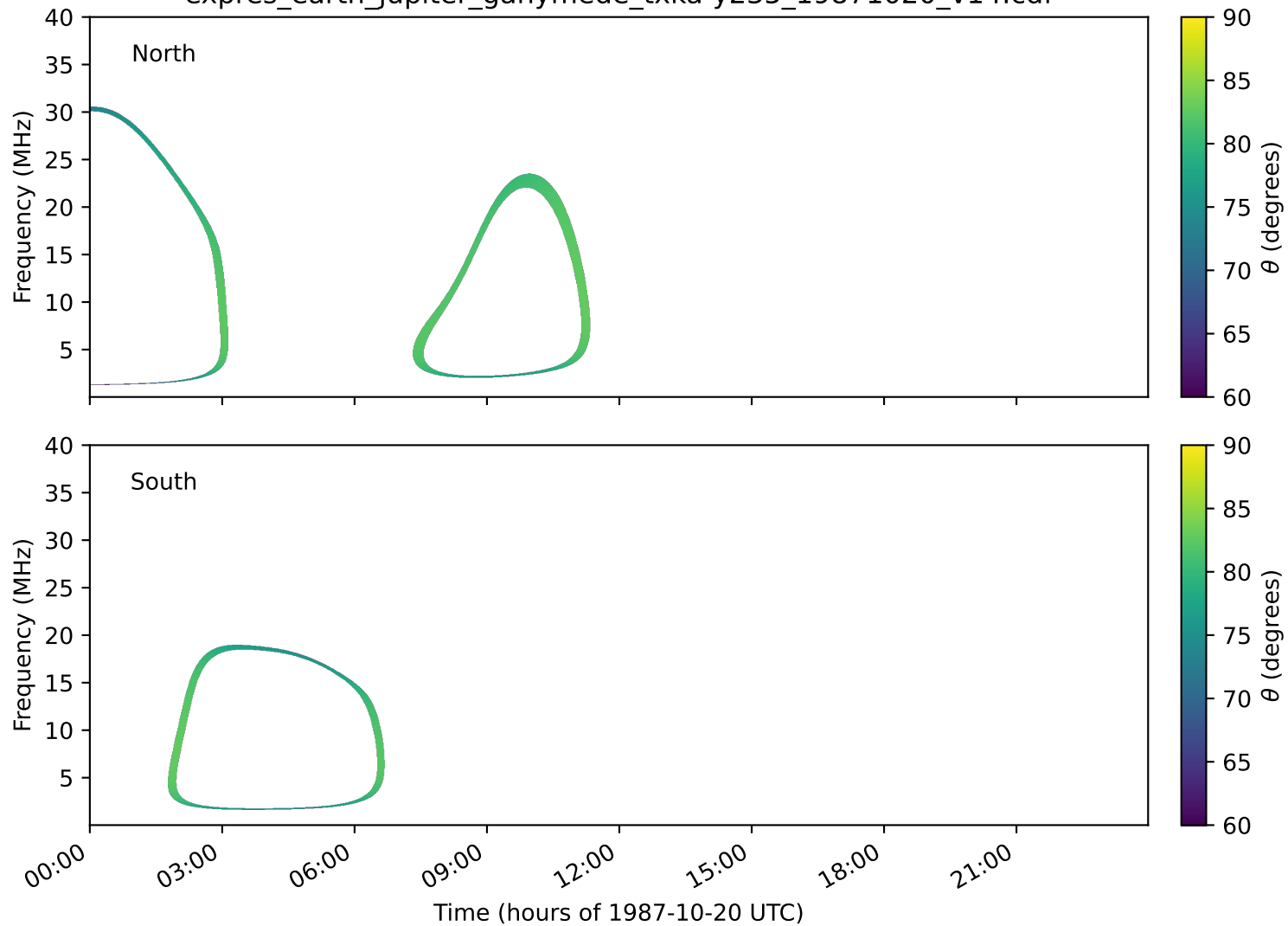
expres_earth_jupiter_ganymede_txka-y235_19871020_v14.cdf
