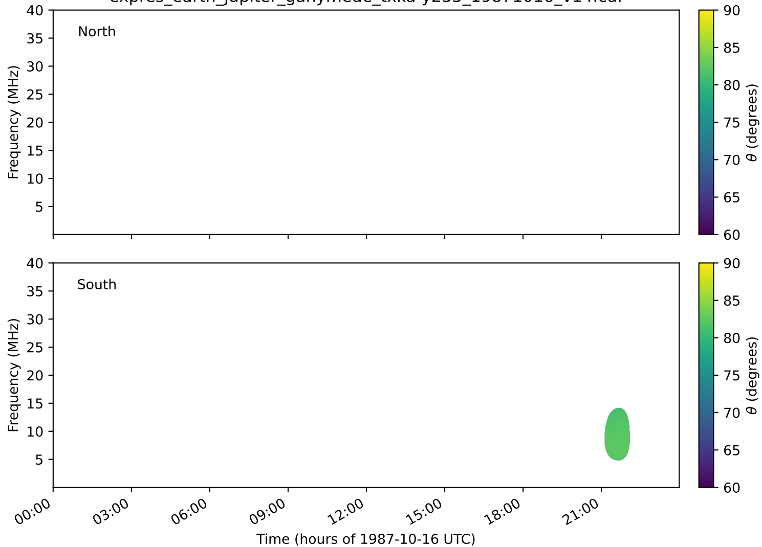
expres_earth_jupiter_ganymede_txka-y235_19871016_v14.cdf
