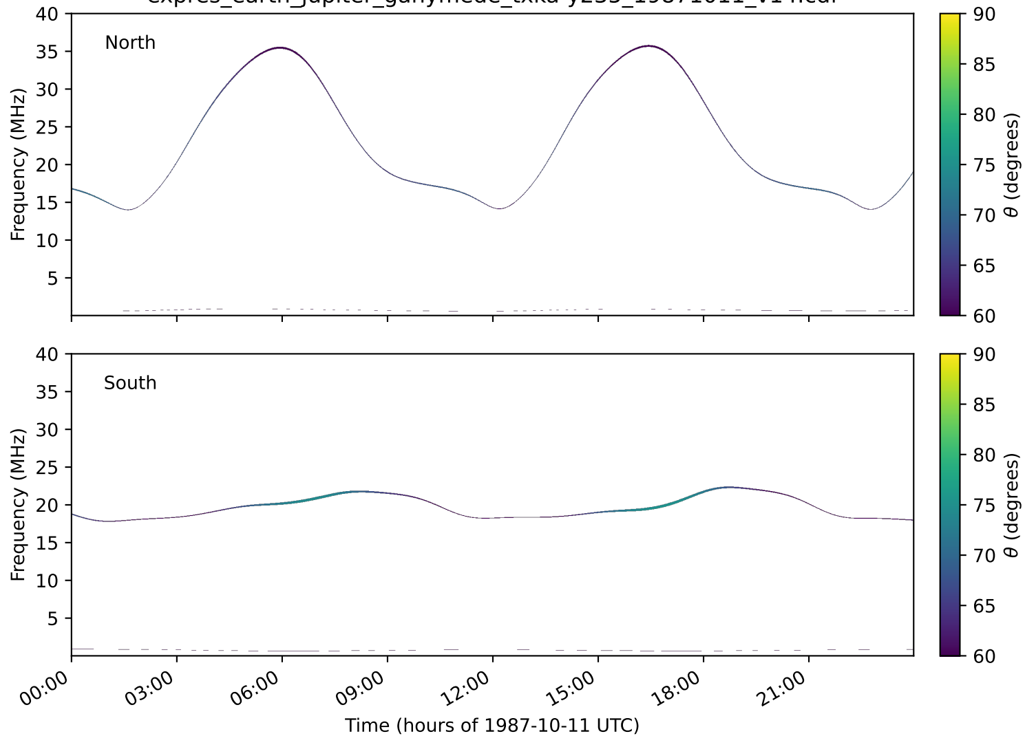
expres_earth_jupiter_ganymede_txka-y235_19871011_v14.cdf
