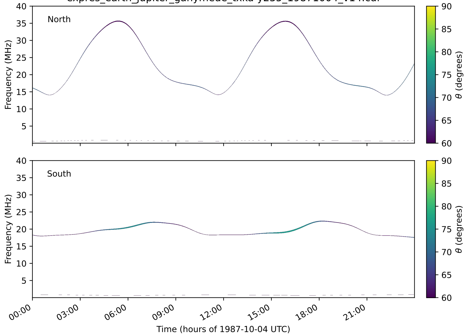
expres_earth_jupiter_ganymede_txka-y235_19871004_v14.cdf
