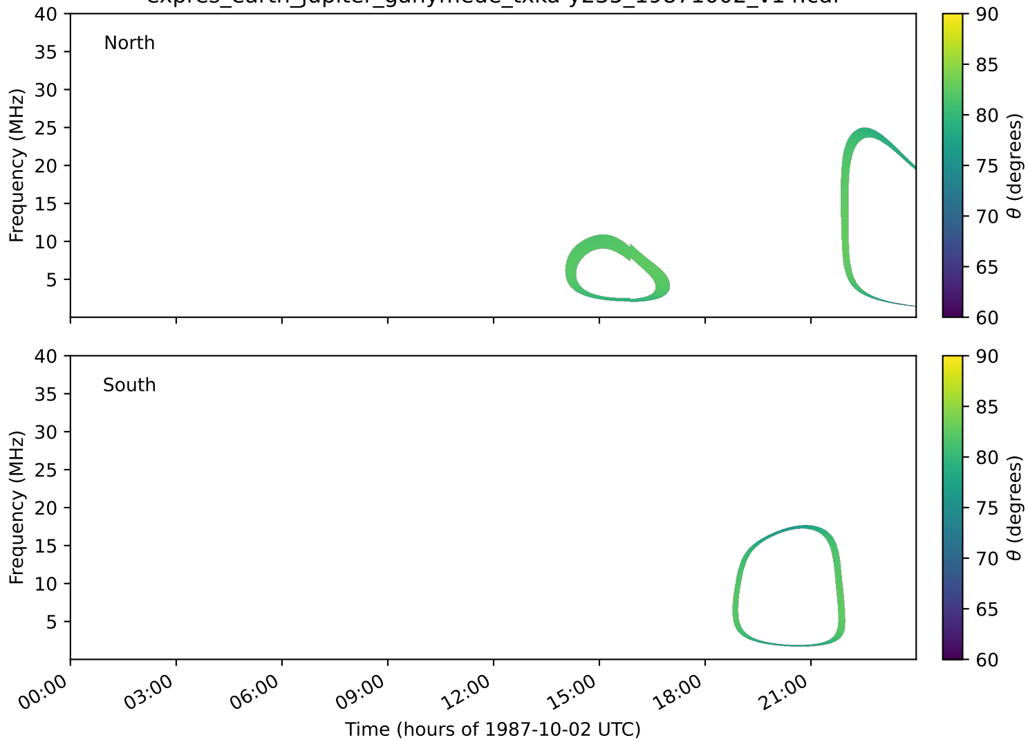
expres_earth_jupiter_ganymede_txka-y235_19871002_v14.cdf
