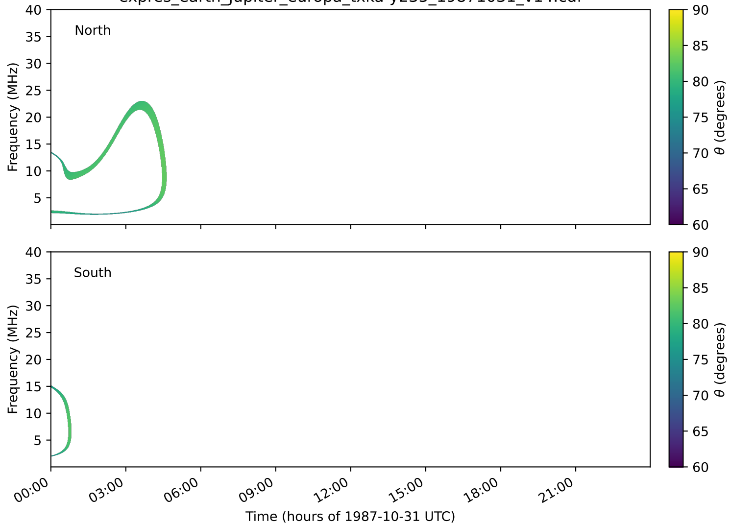
expres_earth_jupiter_europa_txka-y235_19871031_v14.cdf
