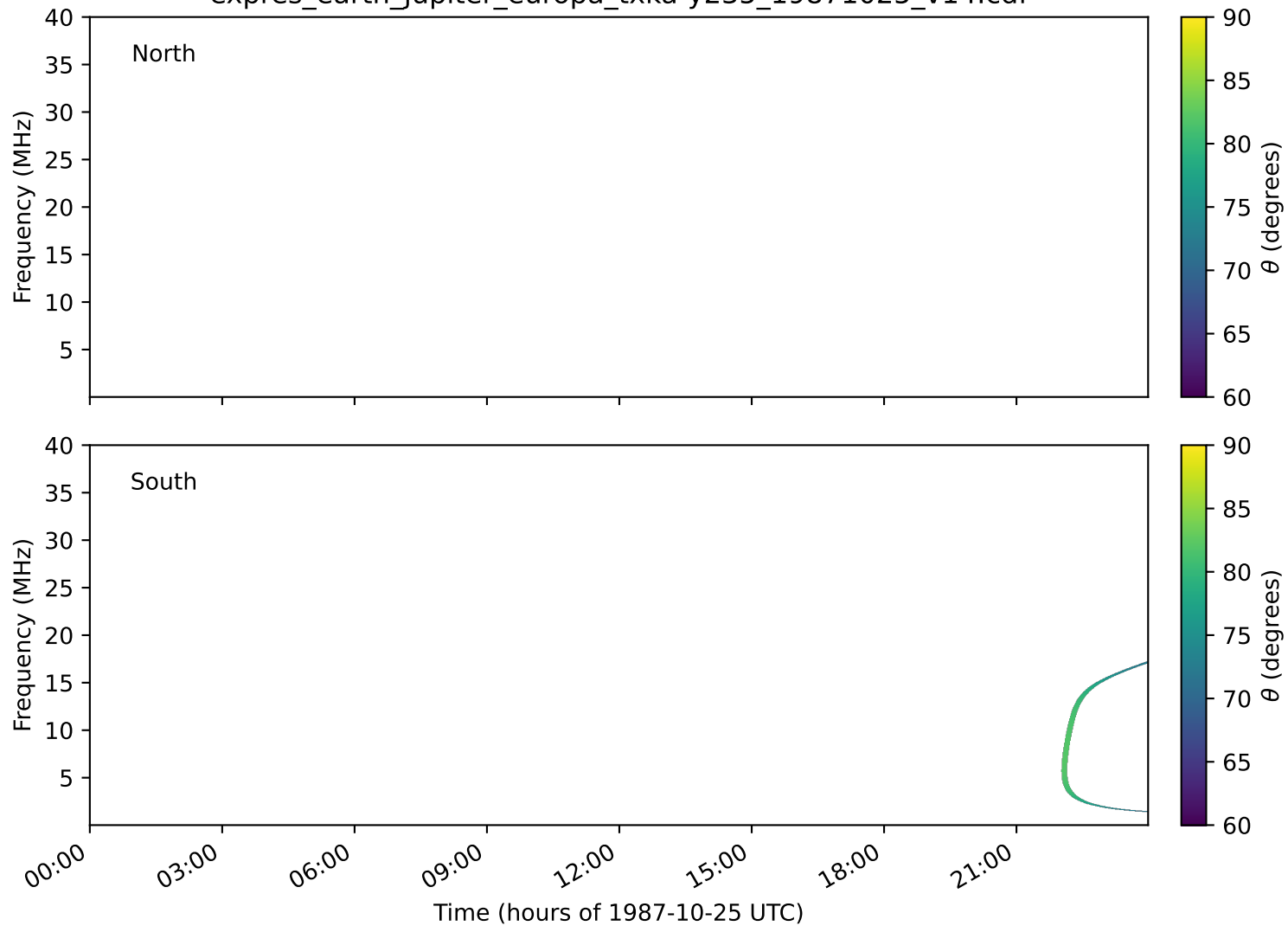
expres_earth_jupiter_europa_txka-y235_19871025_v14.cdf
