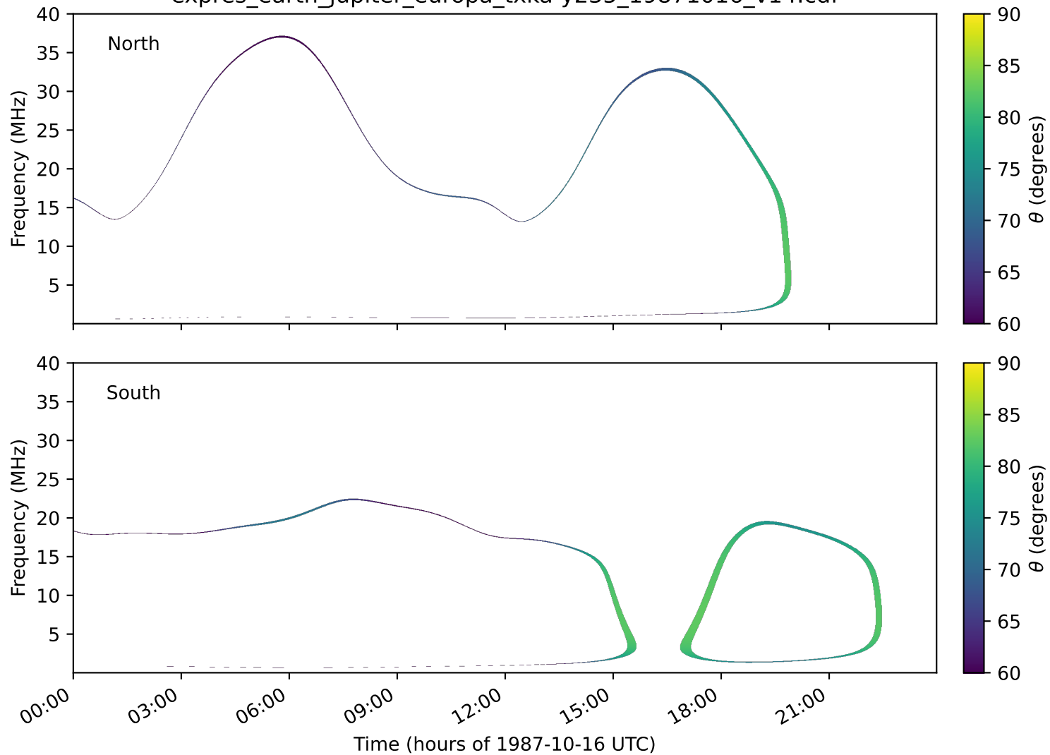
expres_earth_jupiter_europa_txka-y235_19871016_v14.cdf
