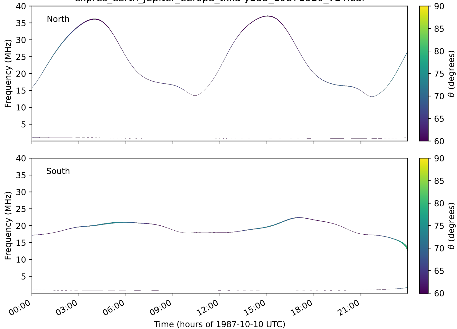
expres_earth_jupiter_europa_txka-y235_19871010_v14.cdf
