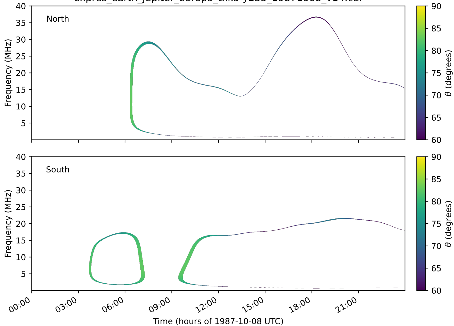
expres_earth_jupiter_europa_txka-y235_19871008_v14.cdf
