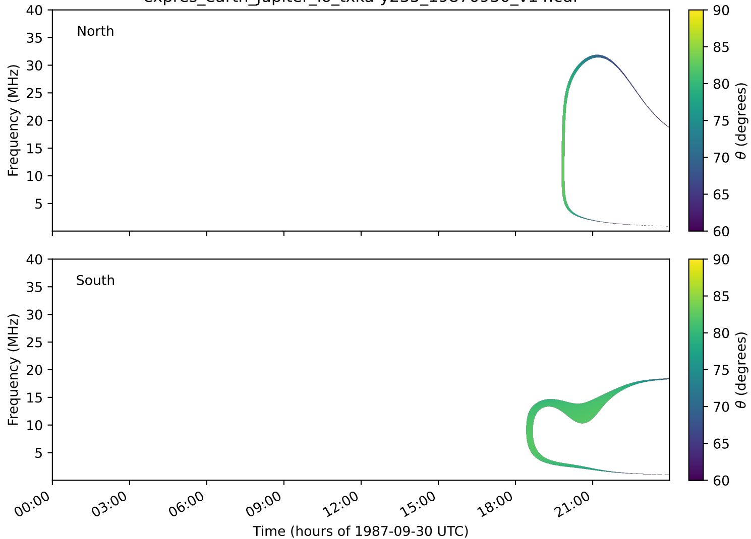
expres_earth_jupiter_io_txka-y235_19870930_v14.cdf
