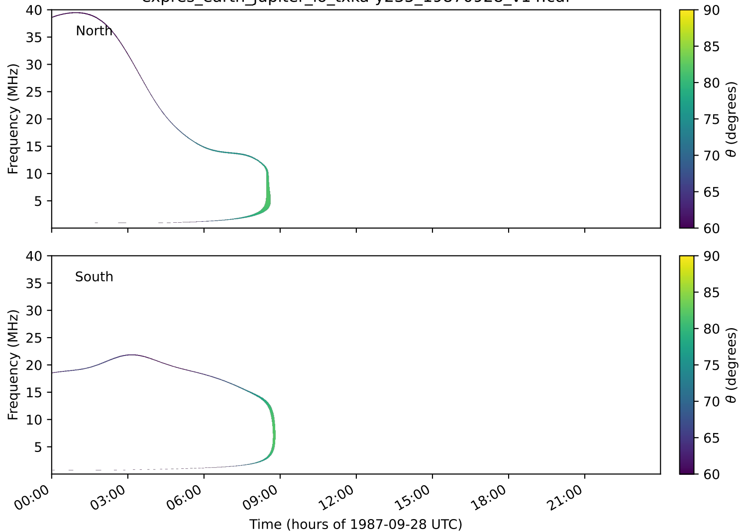
expres_earth_jupiter_io_txka-y235_19870928_v14.cdf
