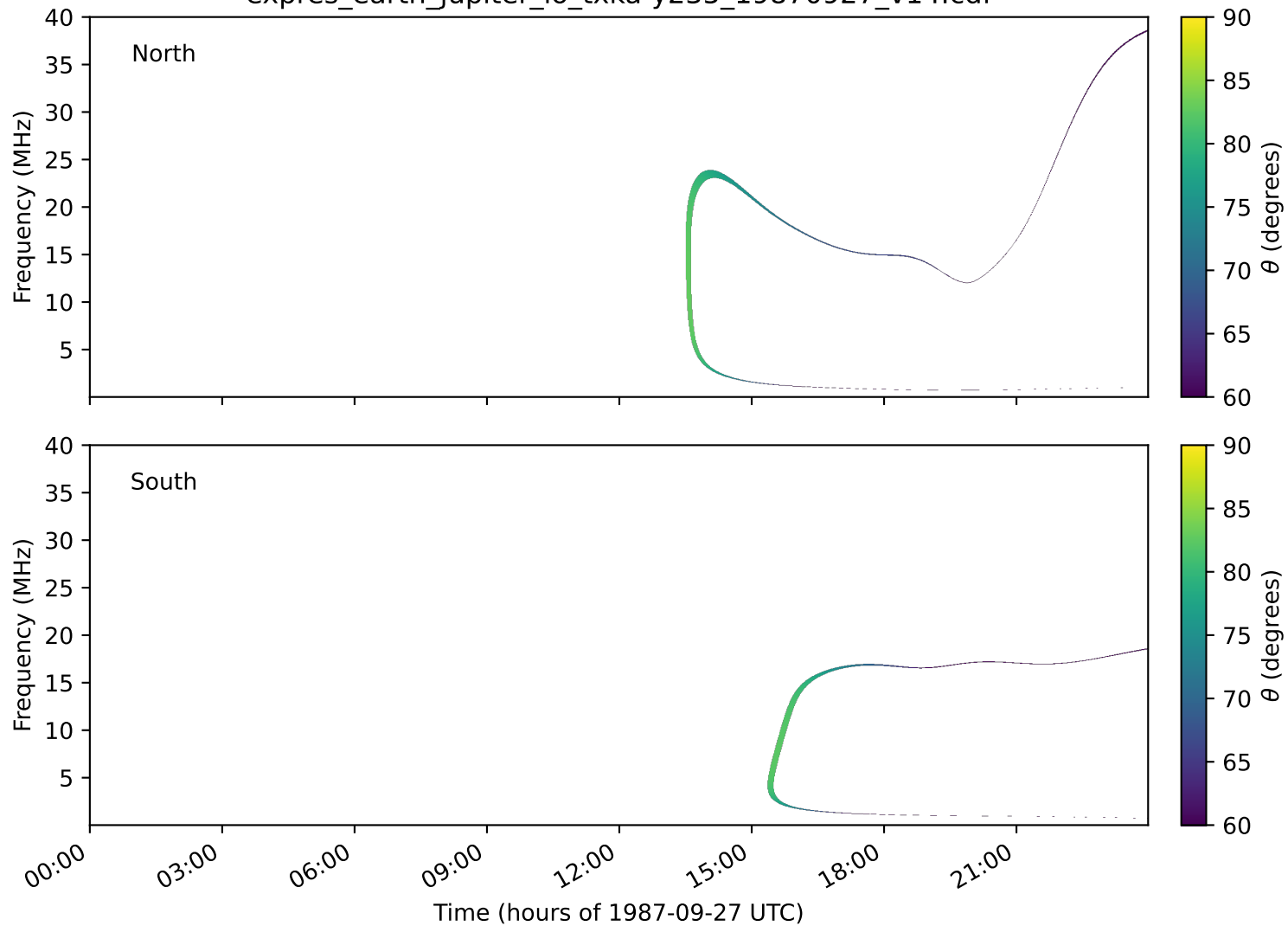
expres_earth_jupiter_io_txka-y235_19870927_v14.cdf
