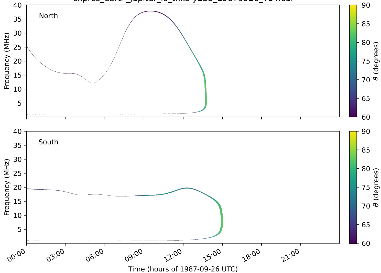
expres_earth_jupiter_io_txka-y235_19870926_v14.cdf
