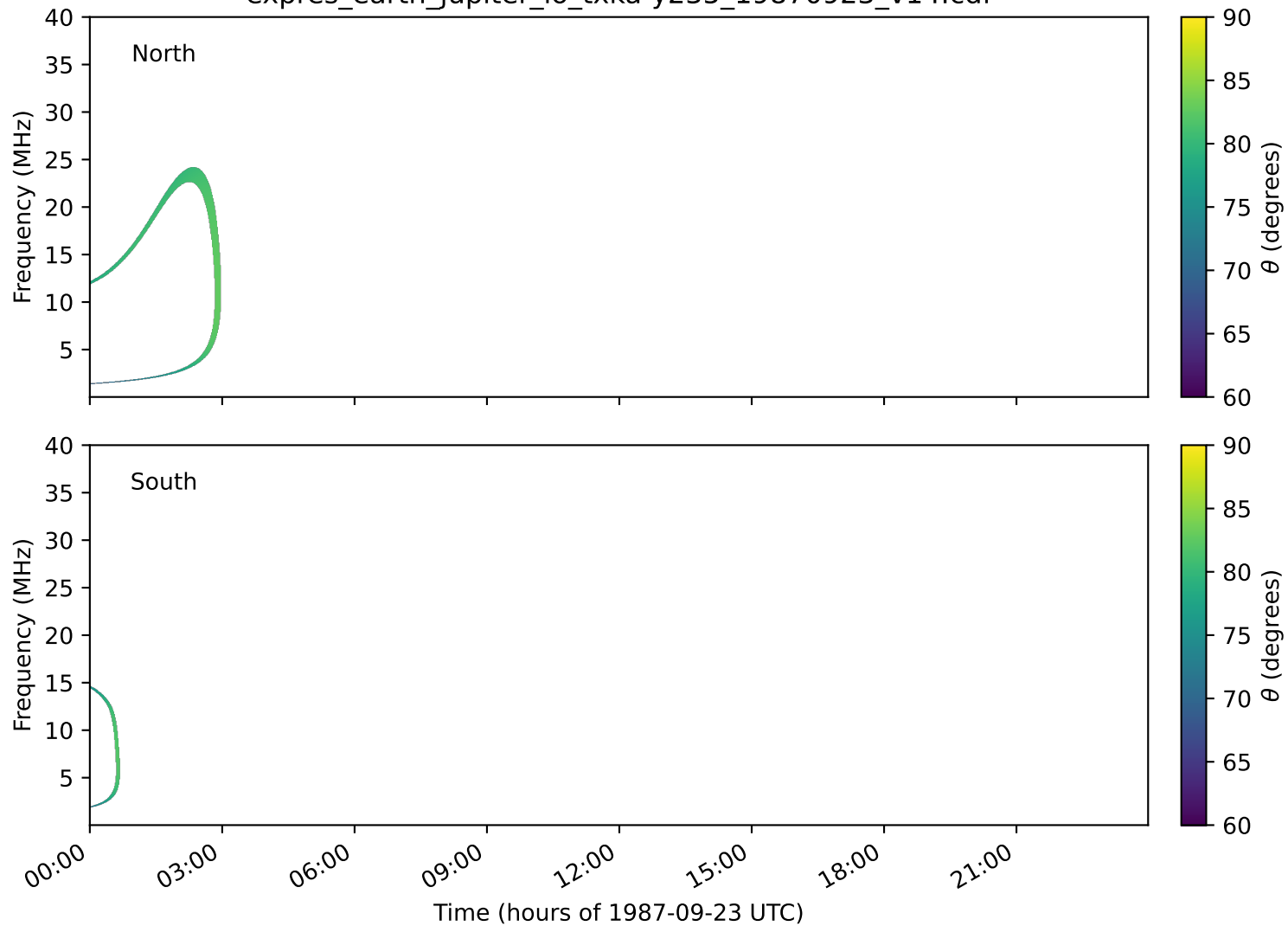
expres_earth_jupiter_io_txka-y235_19870923_v14.cdf
