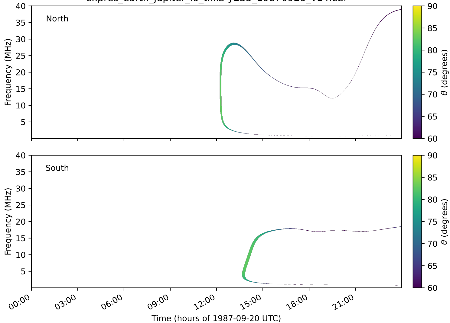
expres_earth_jupiter_io_txka-y235_19870920_v14.cdf
