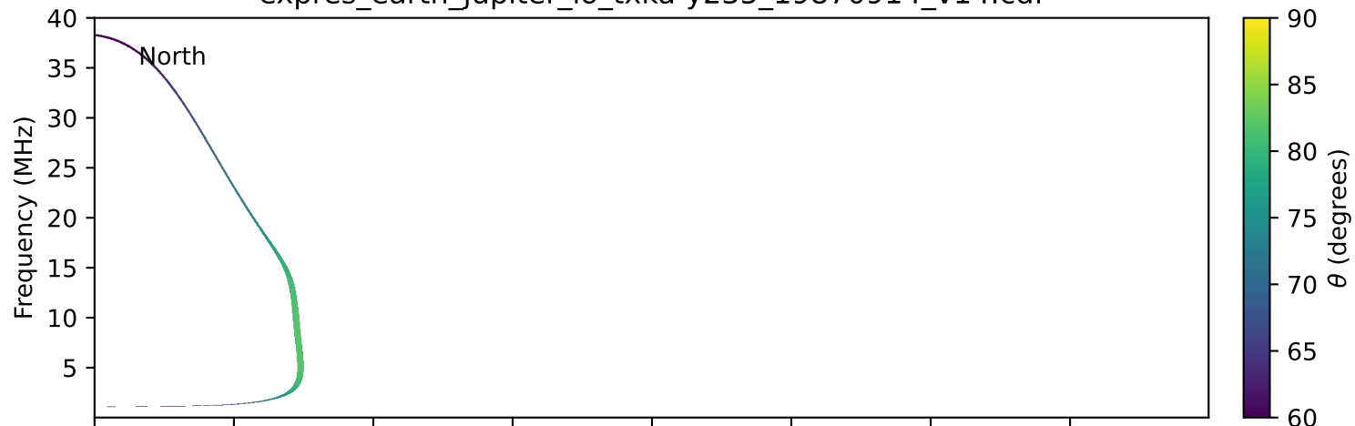
expres_earth_jupiter_io_txka-y235_19870914_v14.cdf
