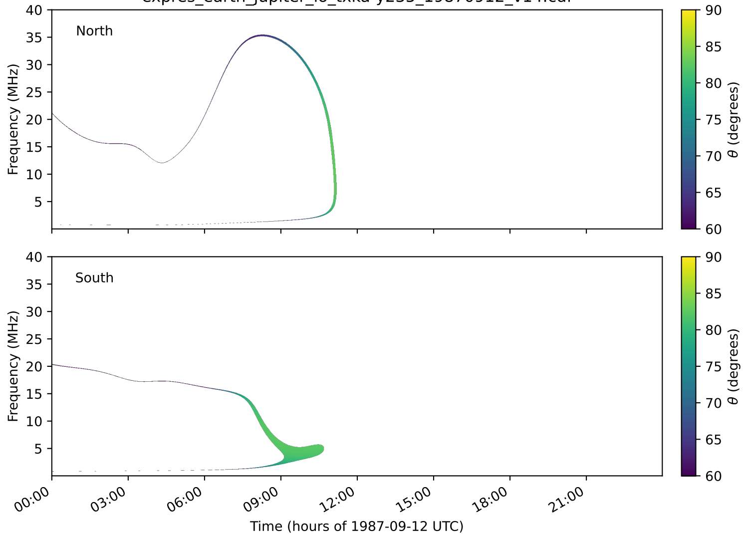
expres_earth_jupiter_io_txka-y235_19870912_v14.cdf
