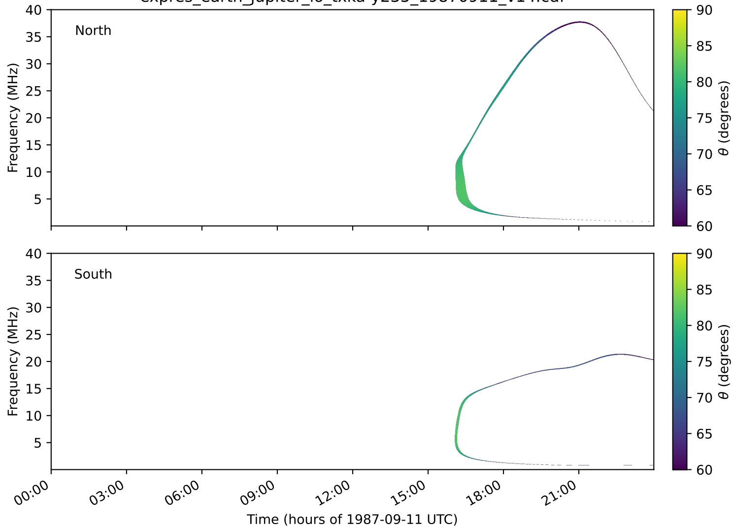
expres_earth_jupiter_io_txka-y235_19870911_v14.cdf
