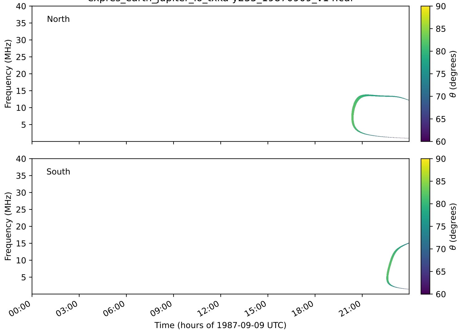
expres_earth_jupiter_io_txka-y235_19870909_v14.cdf
