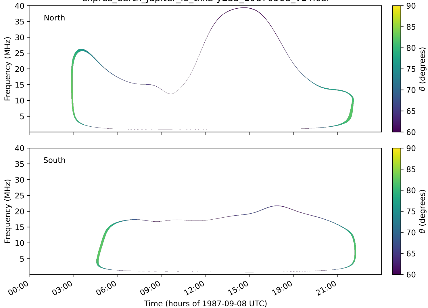
expres_earth_jupiter_io_txka-y235_19870908_v14.cdf
