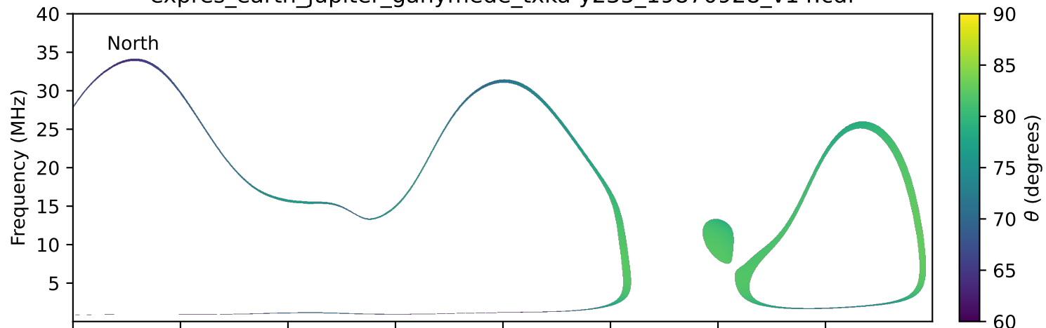
expres_earth_jupiter_ganymede_txka-y235_19870928_v14.cdf
