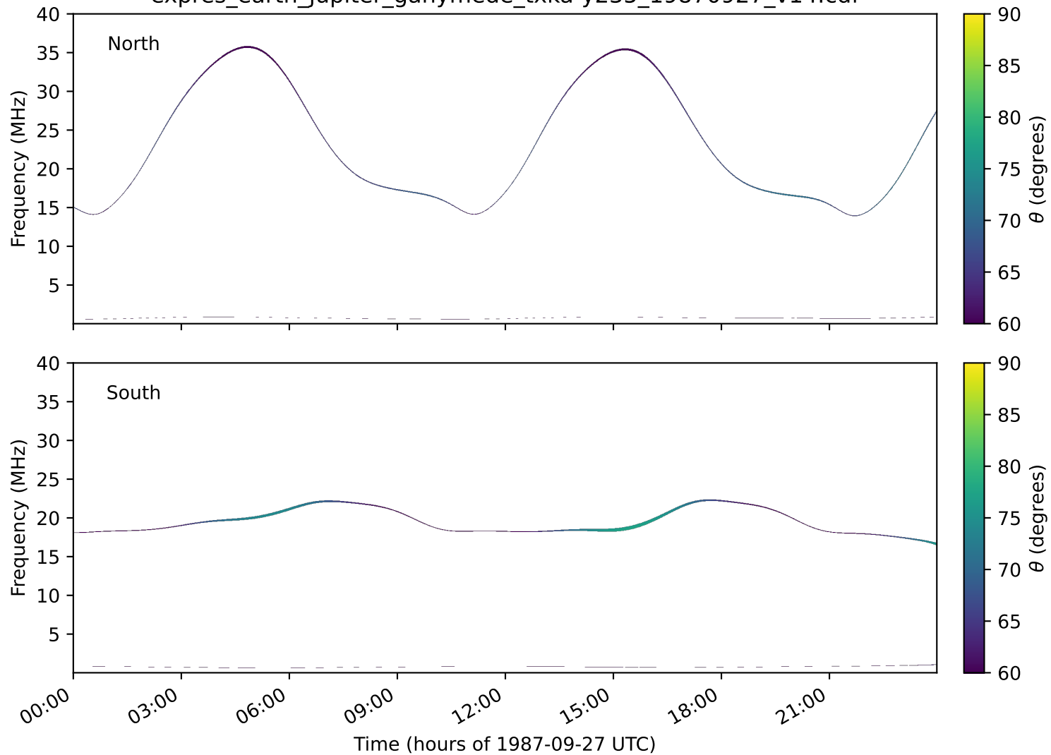
expres_earth_jupiter_ganymede_txka-y235_19870927_v14.cdf
