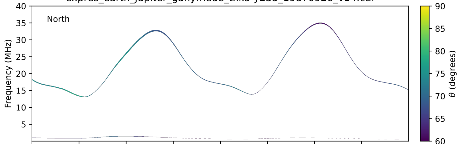
expres_earth_jupiter_ganymede_txka-y235_19870926_v14.cdf
