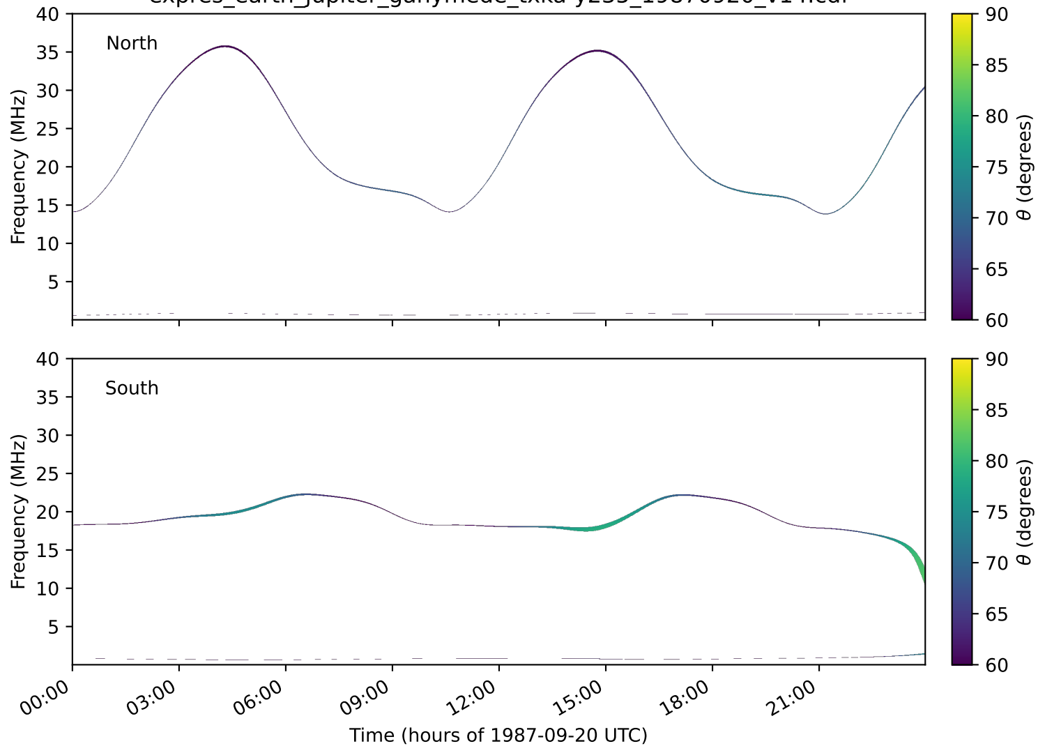
expres_earth_jupiter_ganymede_txka-y235_19870920_v14.cdf
