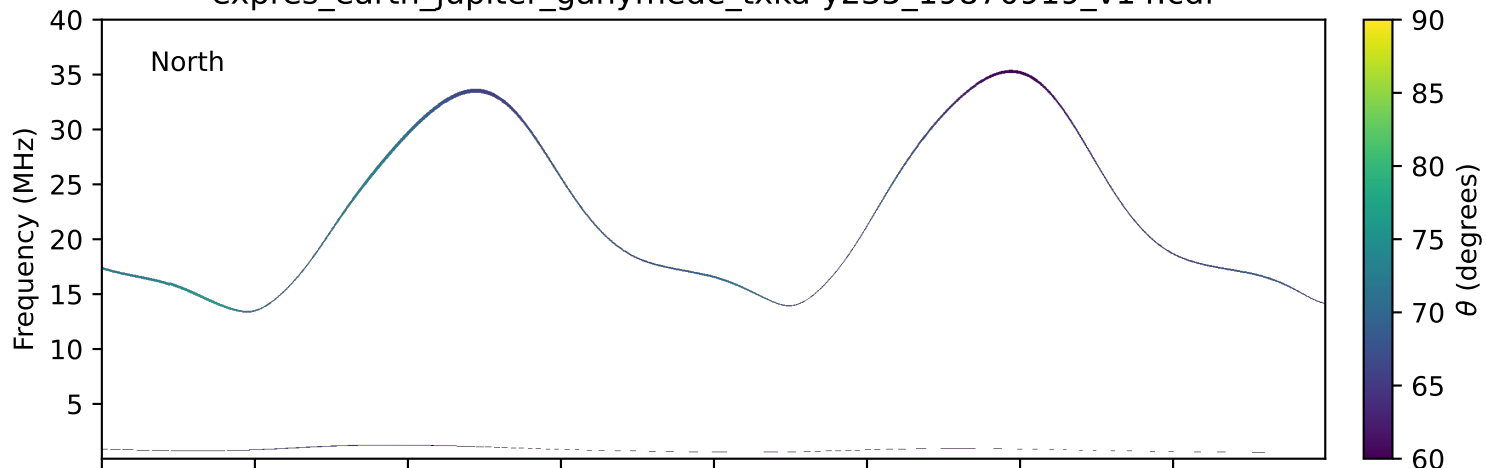
expres_earth_jupiter_ganymede_txka-y235_19870919_v14.cdf
