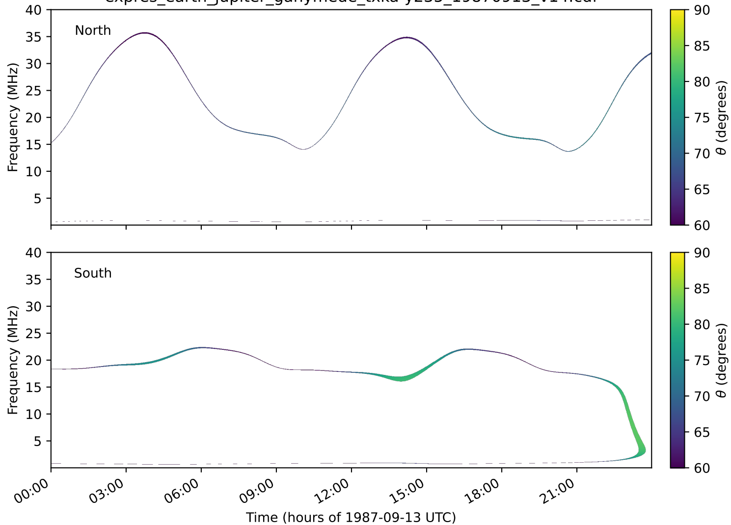
expres_earth_jupiter_ganymede_txka-y235_19870913_v14.cdf
