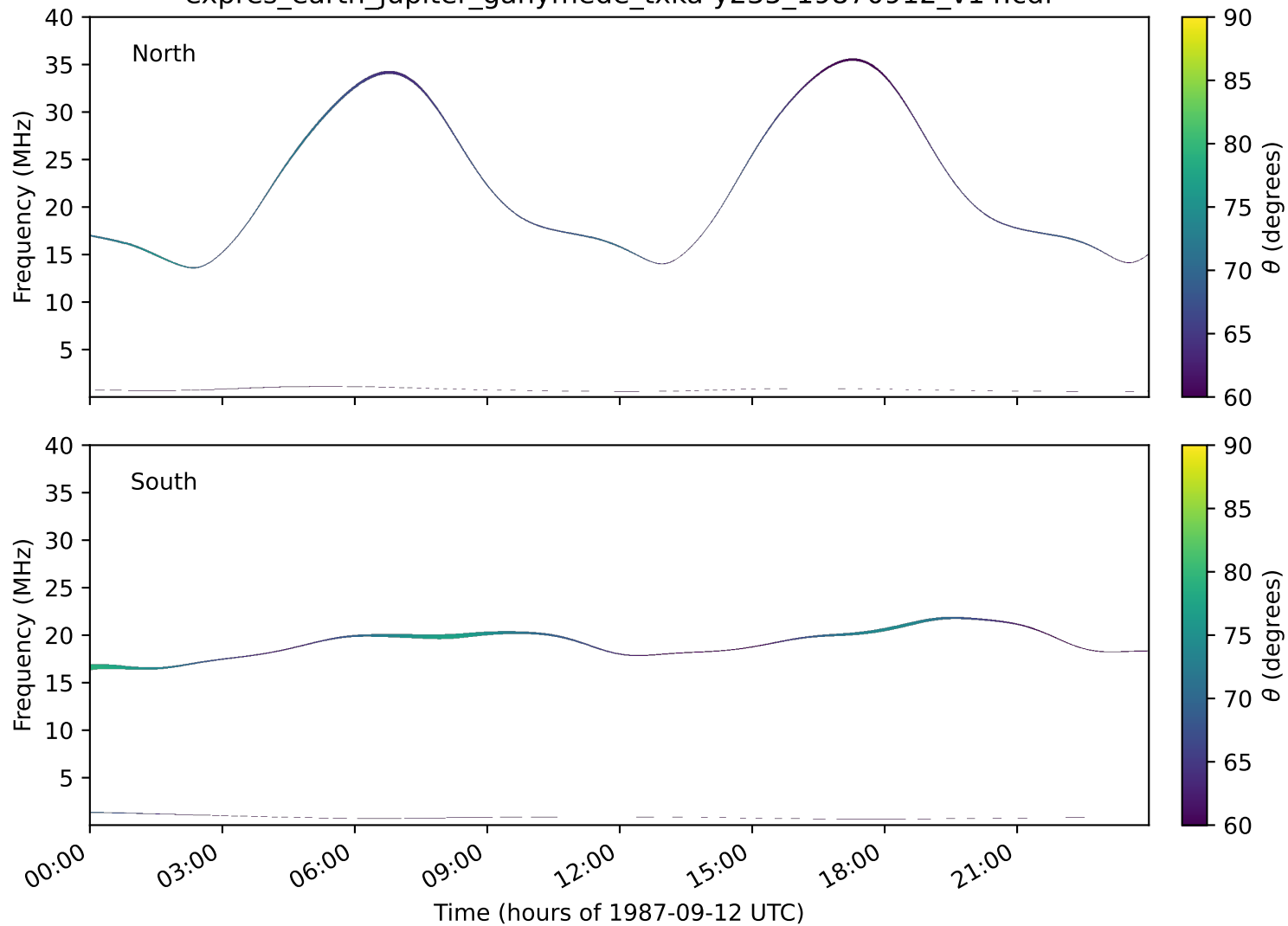
expres_earth_jupiter_ganymede_txka-y235_19870912_v14.cdf
