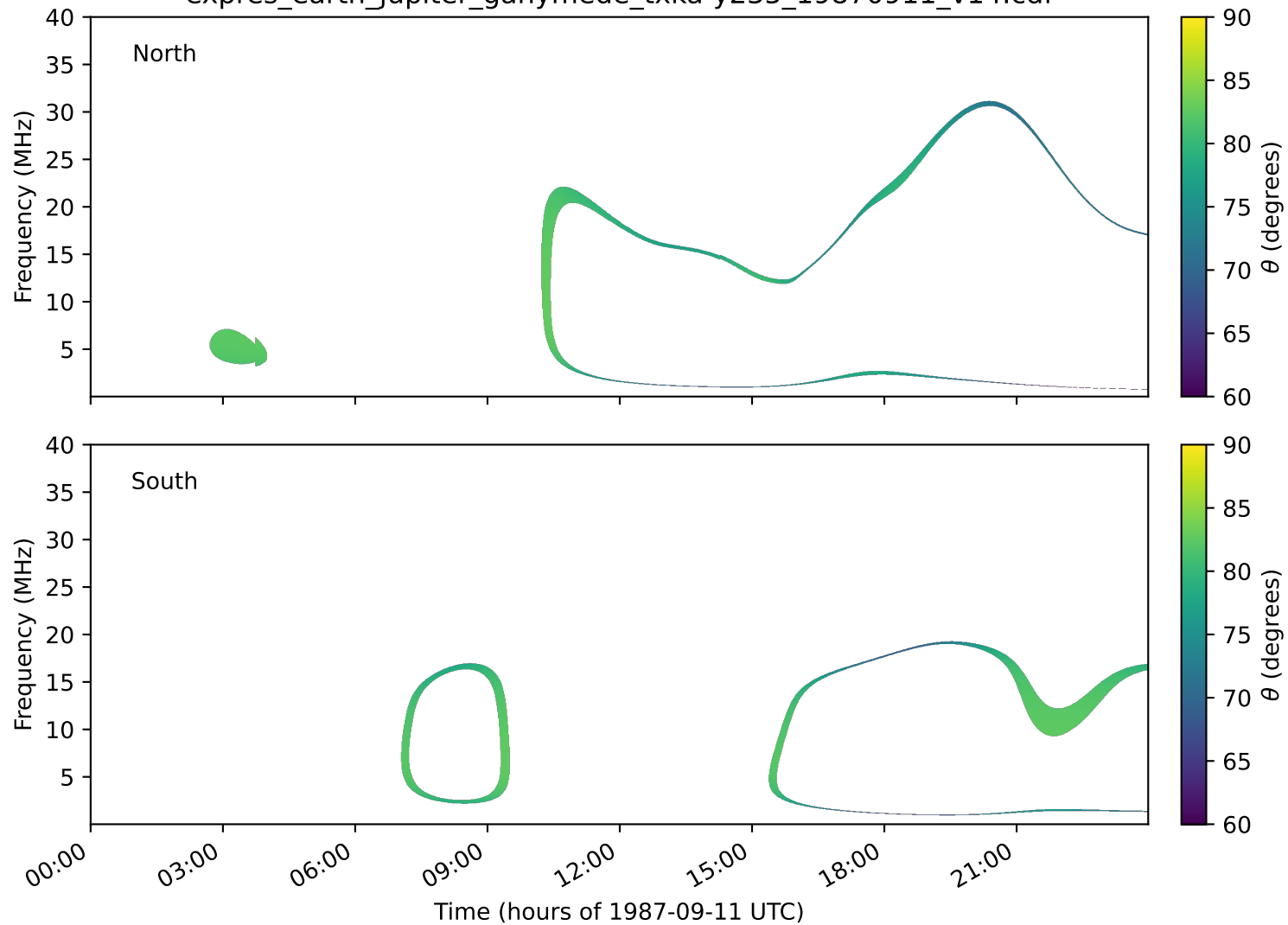
expres_earth_jupiter_ganymede_txka-y235_19870911_v14.cdf
