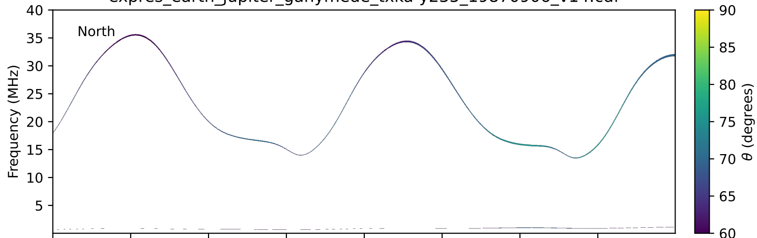
expres_earth_jupiter_ganymede_txka-y235_19870906_v14.cdf
