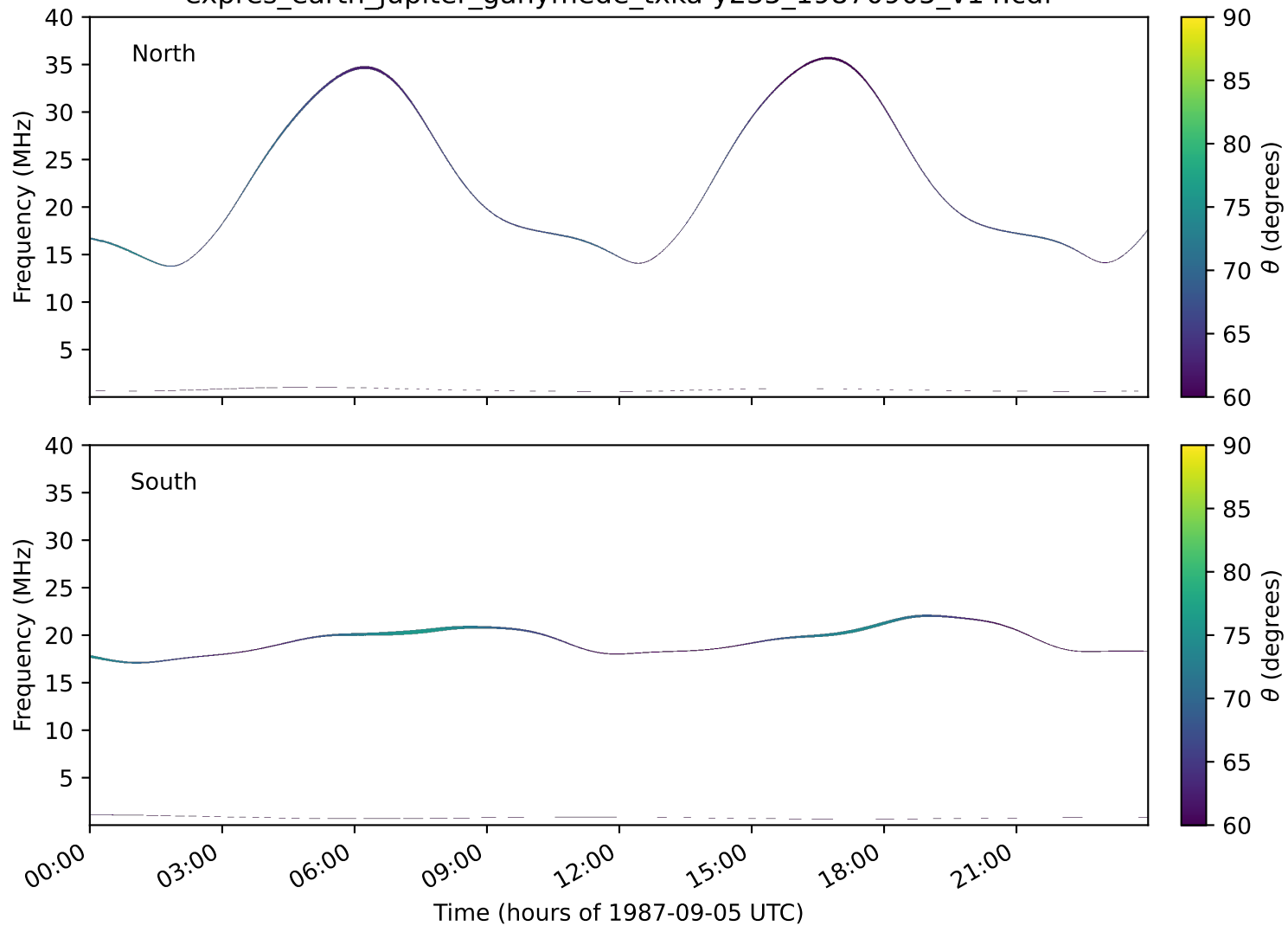
expres_earth_jupiter_ganymede_txka-y235_19870905_v14.cdf
