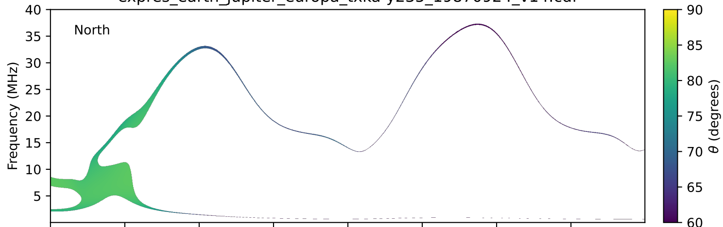
expres_earth_jupiter_europa_txka-y235_19870924_v14.cdf
