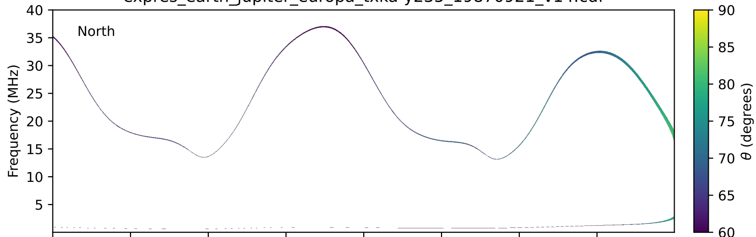
expres_earth_jupiter_europa_txka-y235_19870921_v14.cdf
