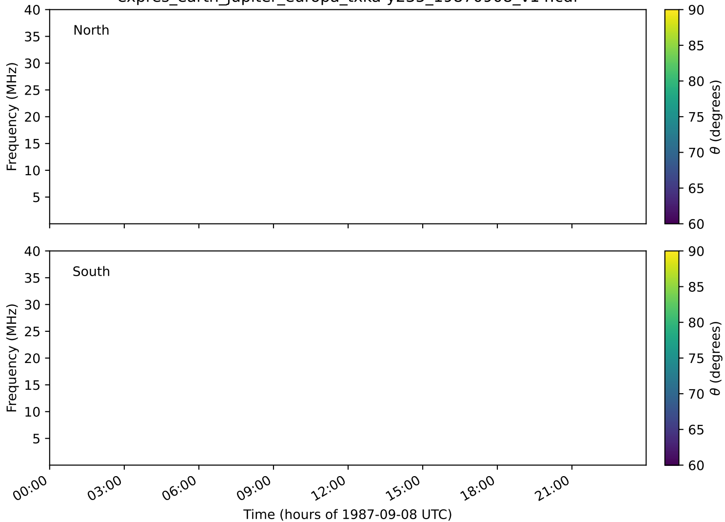
expres_earth_jupiter_europa_txka-y235_19870908_v14.cdf
