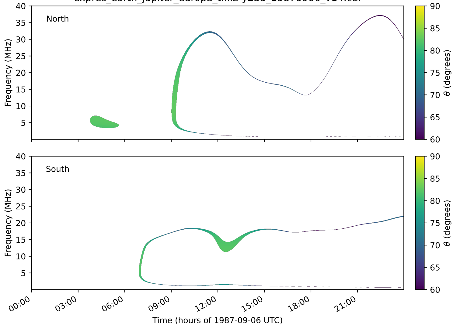
expres_earth_jupiter_europa_txka-y235_19870906_v14.cdf
