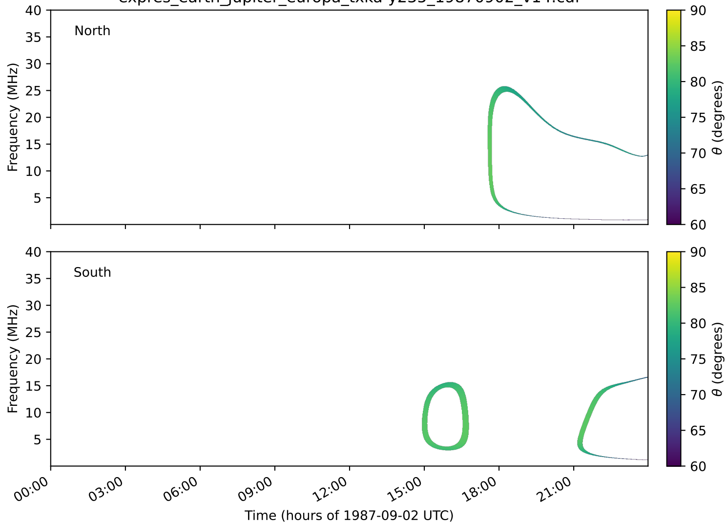
expres_earth_jupiter_europa_txka-y235_19870902_v14.cdf
