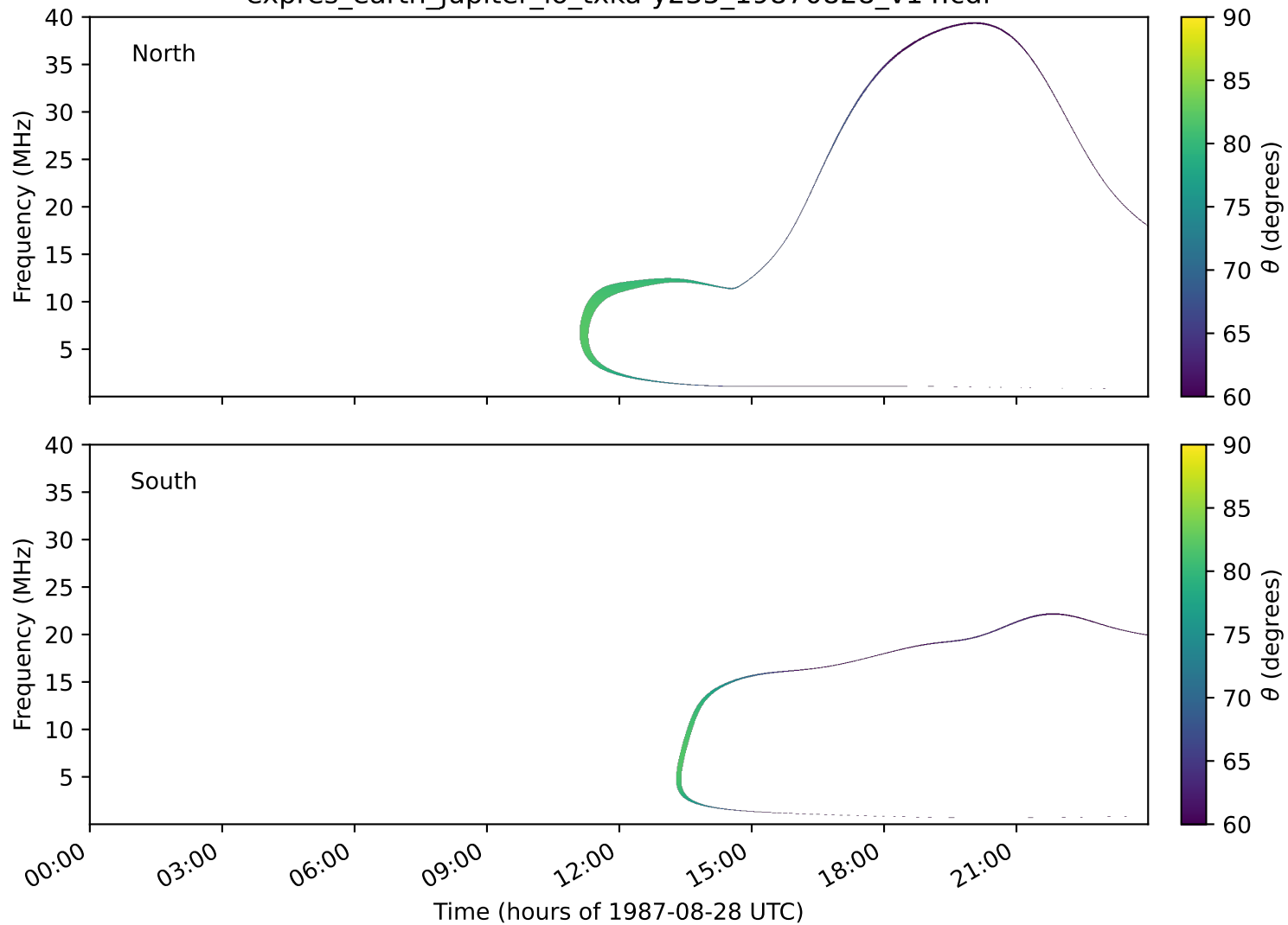
expres_earth_jupiter_io_txka-y235_19870828_v14.cdf
