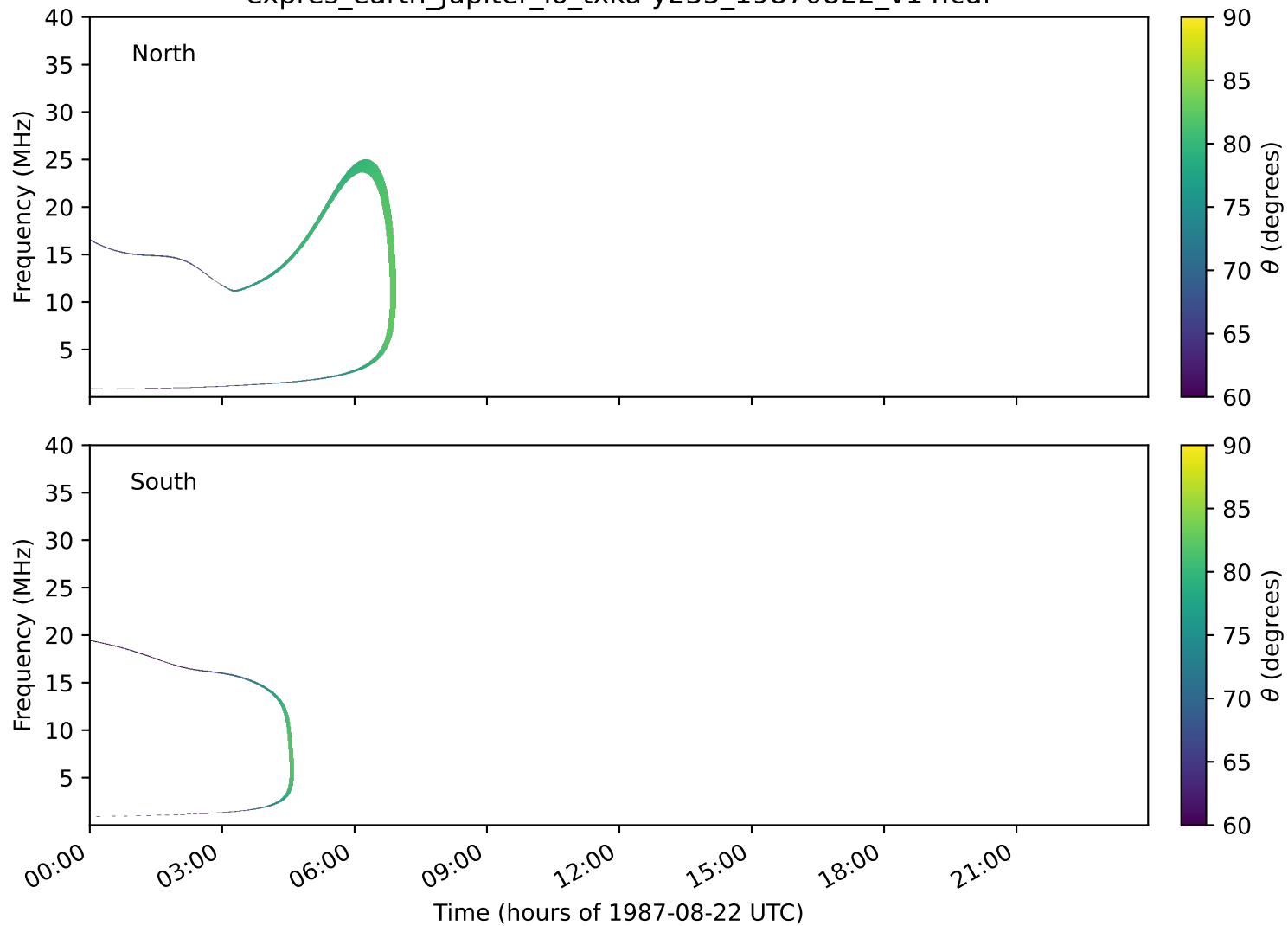
expres_earth_jupiter_io_txka-y235_19870822_v14.cdf
