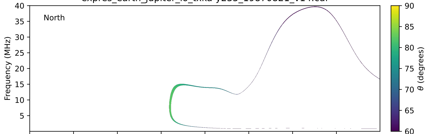
expres_earth_jupiter_io_txka-y235_19870821_v14.cdf
