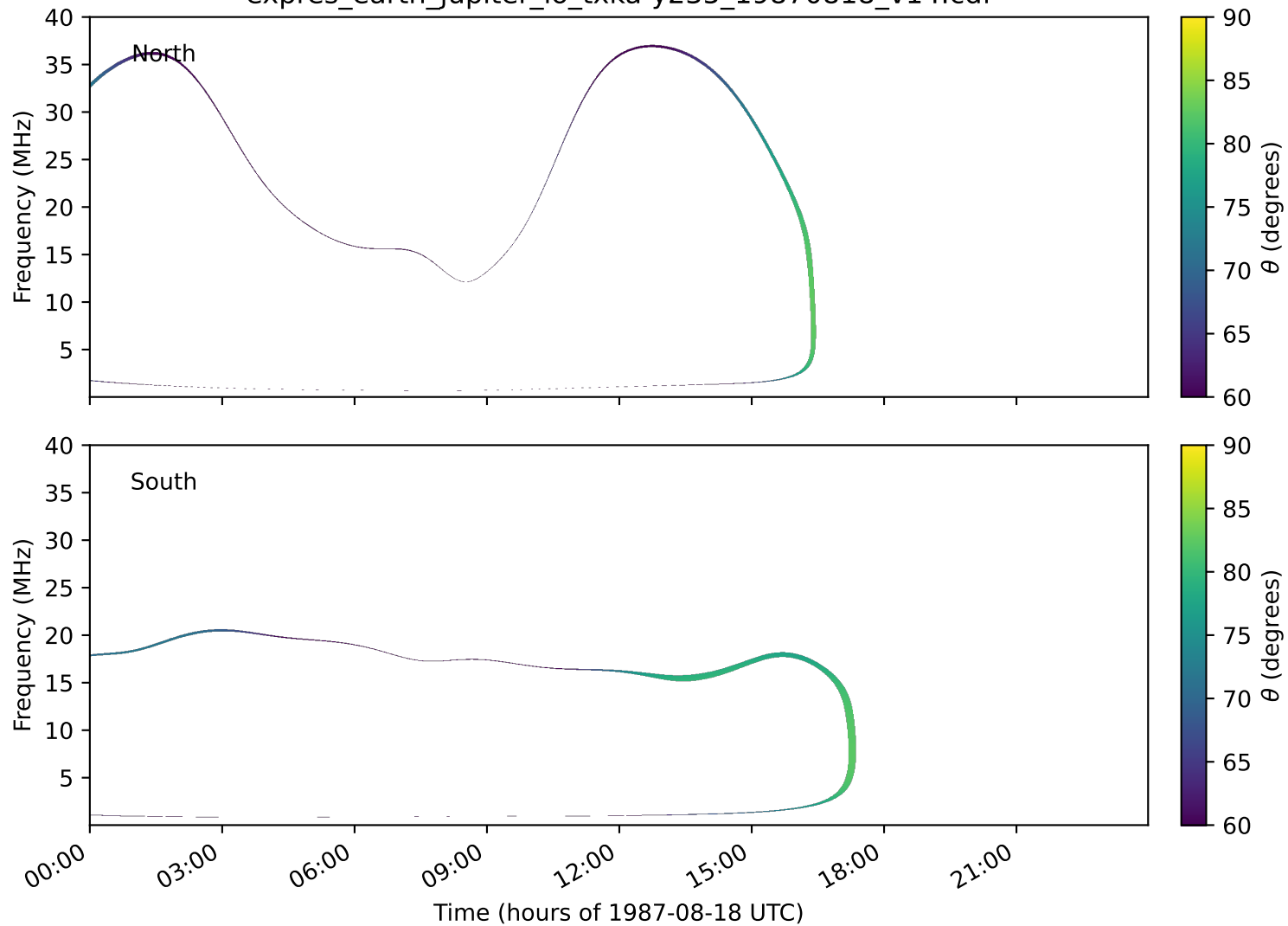
expres_earth_jupiter_io_txka-y235_19870818_v14.cdf
