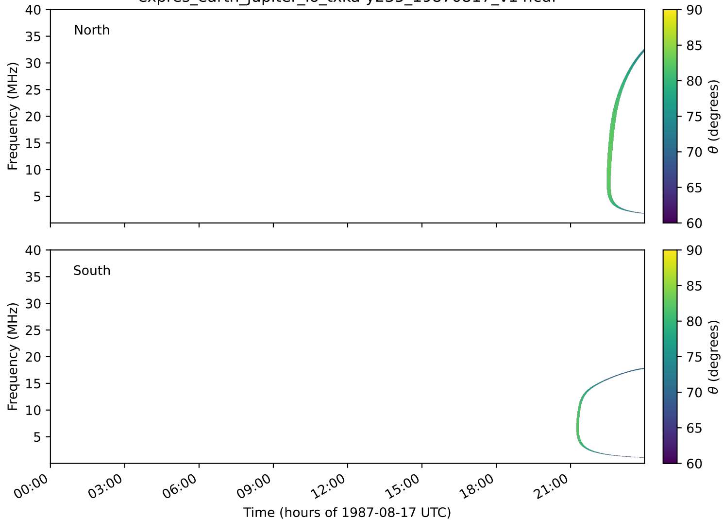
expres_earth_jupiter_io_txka-y235_19870817_v14.cdf
